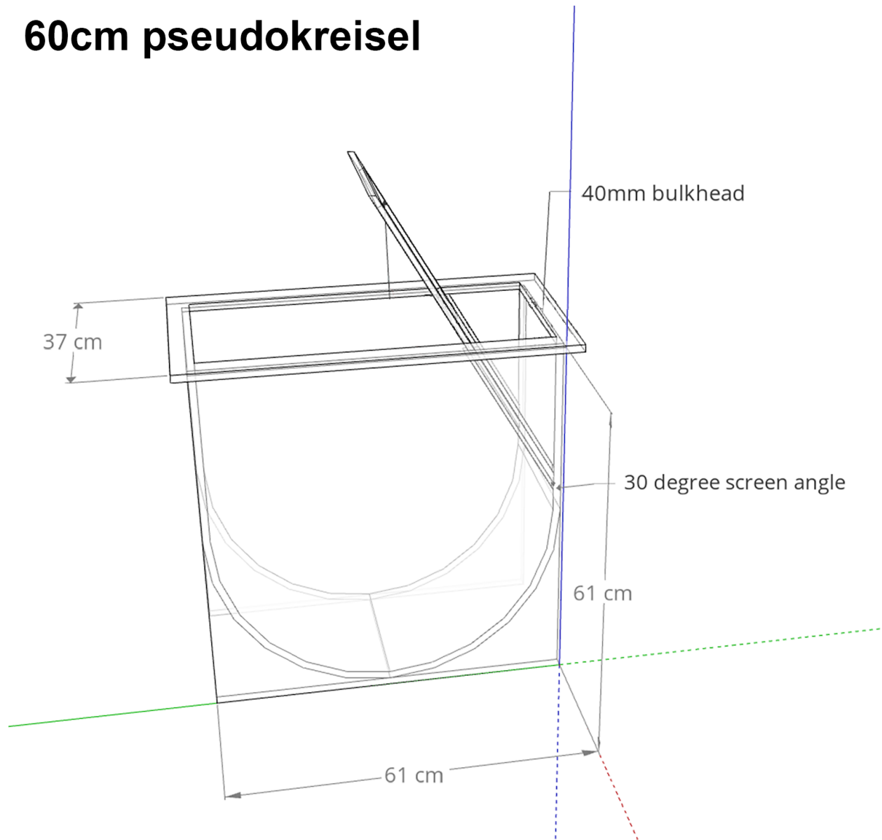
Supplementary Figure 2 | Schematic for ~60 cm basic pseudokreisel design.
