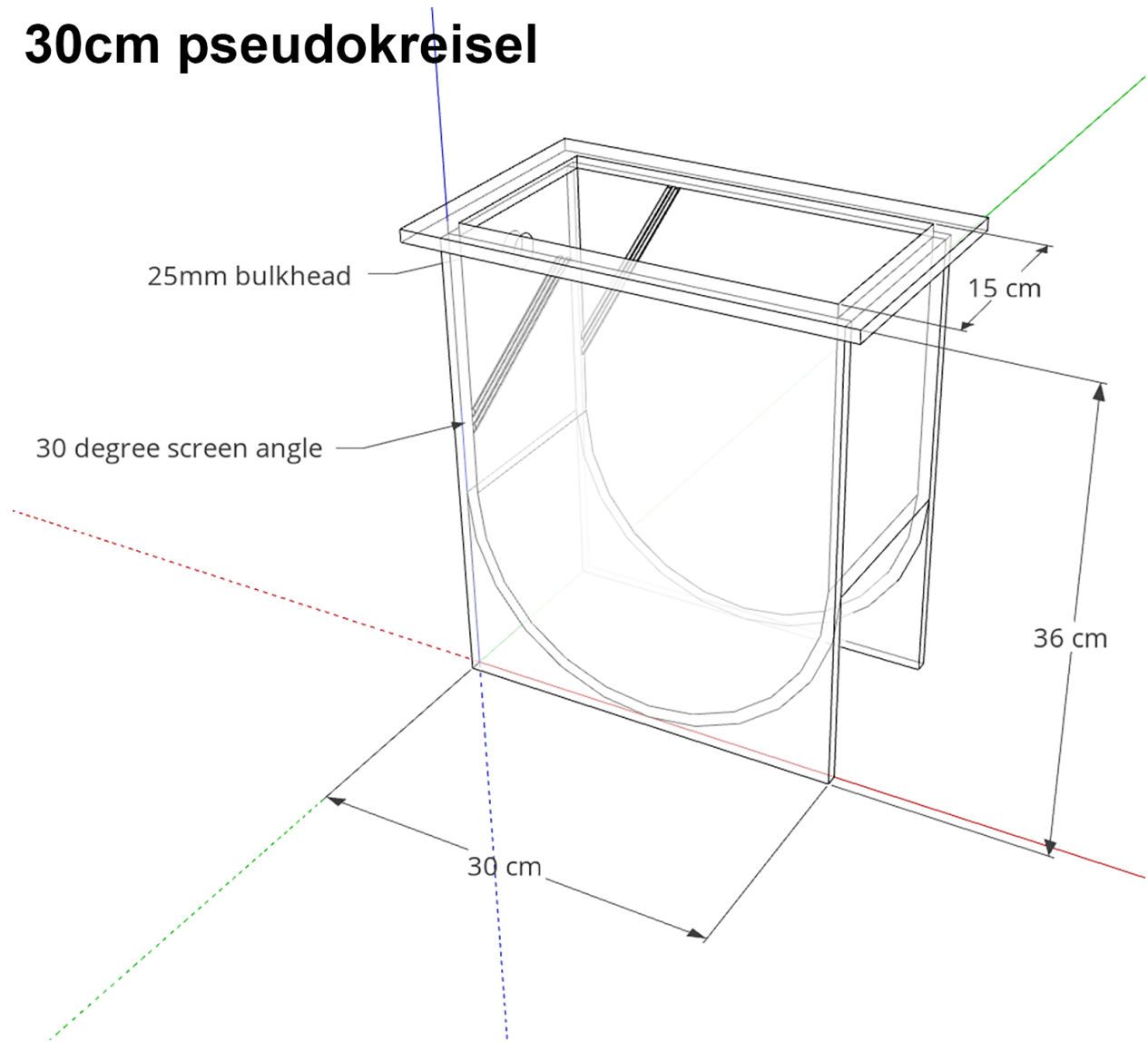
Supplementary Figure 1 | Schematic for ~30 cm basic pseudokreisel design.
